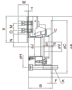
MODEL BBC 3-JAW WEDGE TYPE POWER CHUCK
